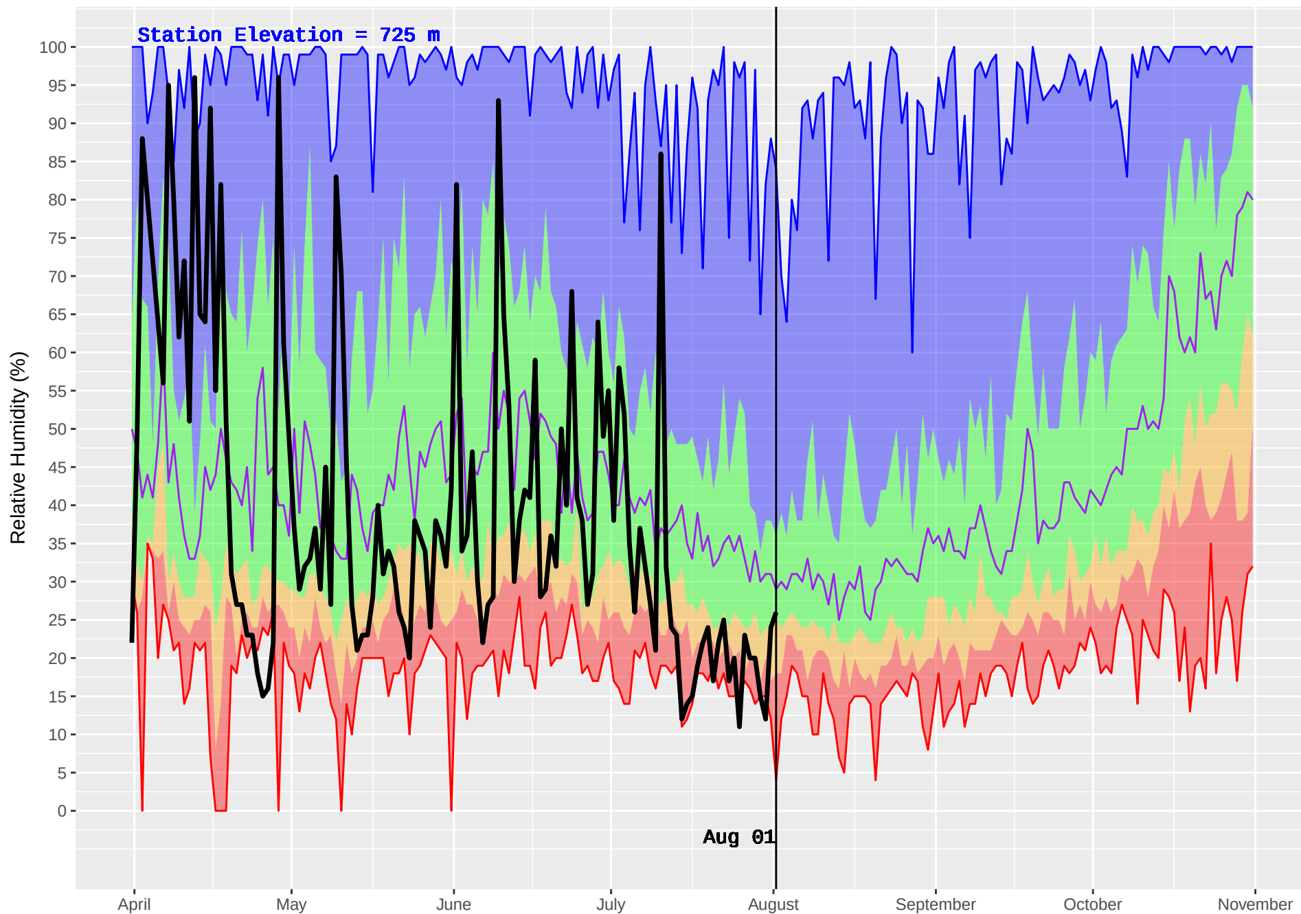
PENDOREILLE (402) : Historical (1986–2016) and Current (2018) Daily Relative Humidity
