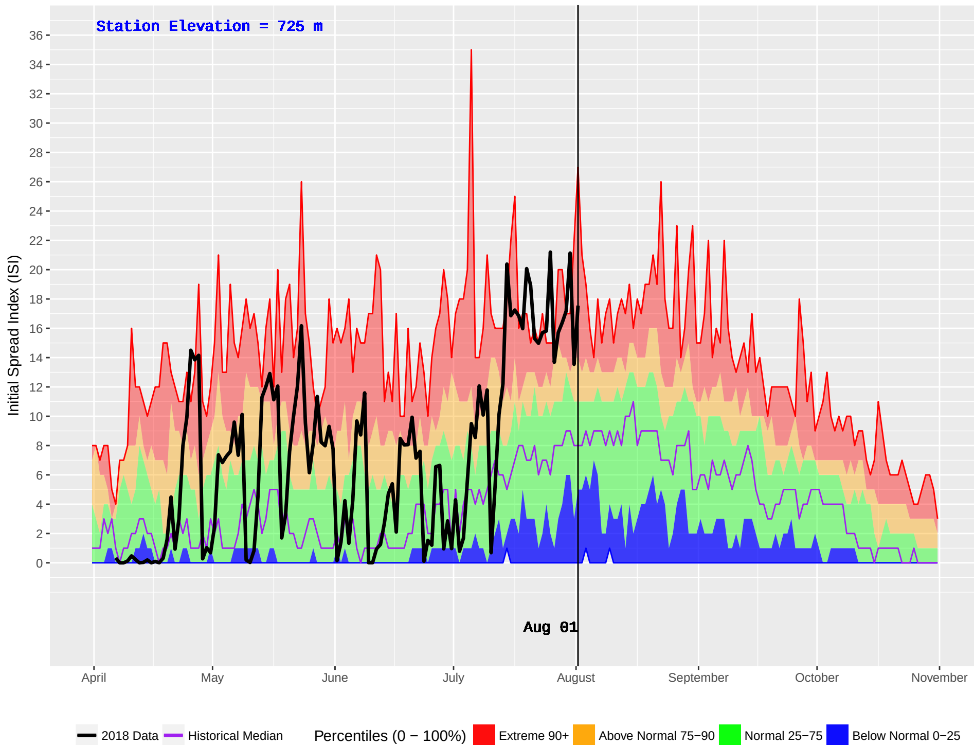
PENDOREILLE (402) : Historical (1986–2016) and Current (2018) Daily Initial Spread Index (ISI)
