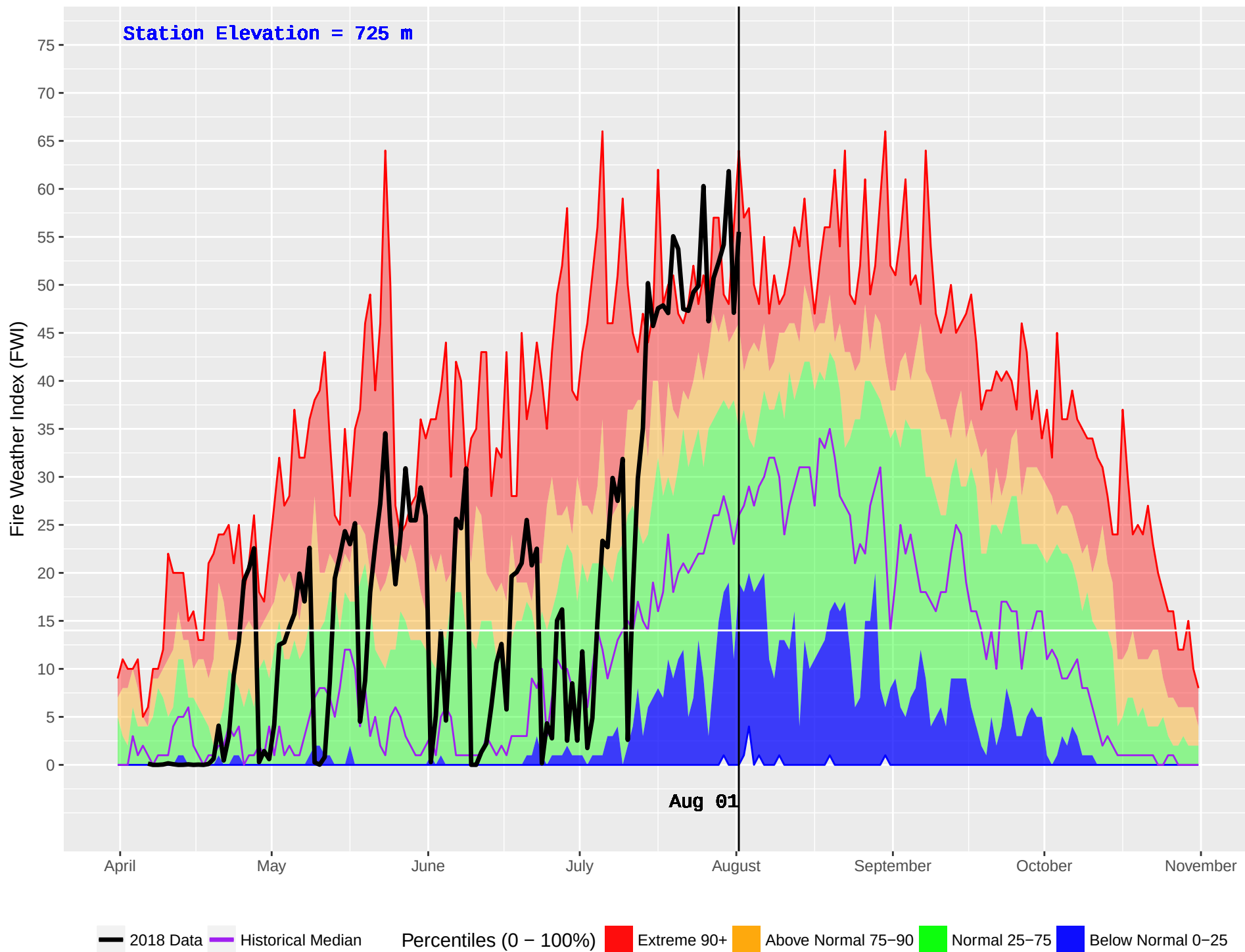
PENDOREILLE (402) : Historical (1986–2016) and Current (2018) Daily Fire Weather Index (FWI)
